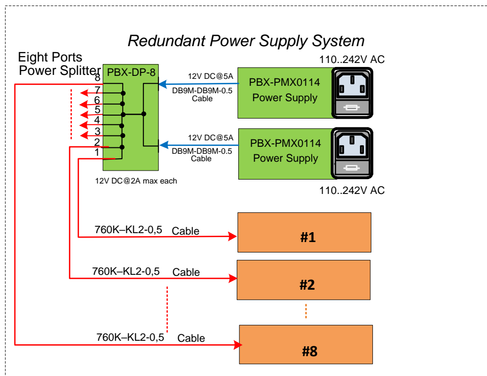
Power supply system with redundancy.
